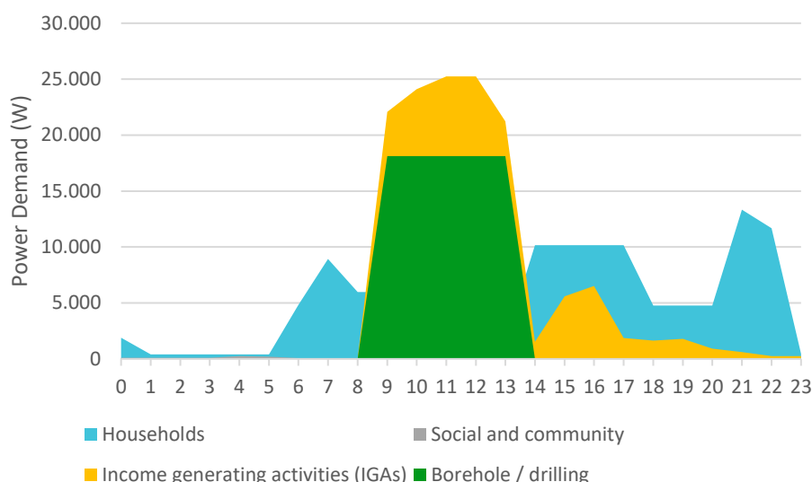
Figure 20: Daily Hourly Load Profile 3 for a Typical Village (more than 1000 inhabitants) in Senegal.
