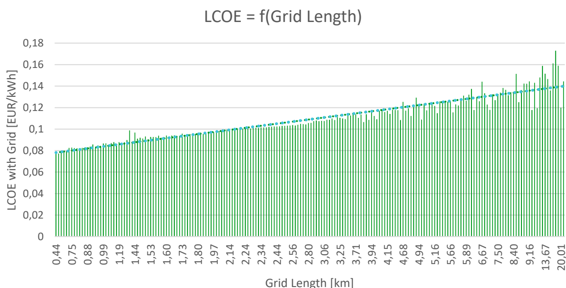
Figure 31: LCOE as a function of Grid Length in Benin (Diesel Share 24.7%, grid investment cost considered)
